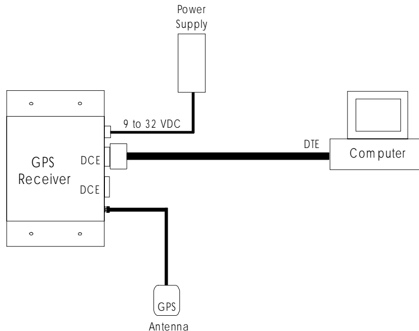
Figure 1-10. Interconnect Diagram
