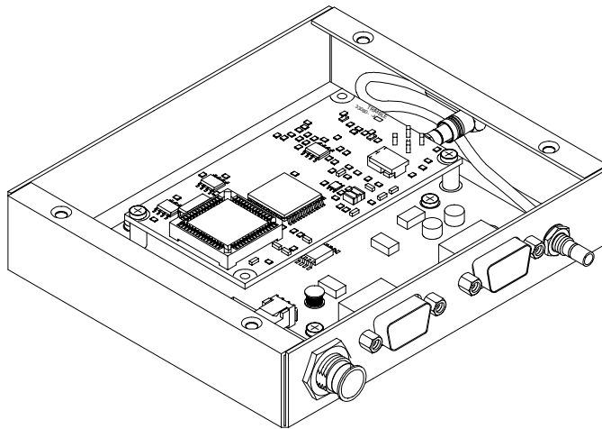
Figure 1-1. The Module Installed Inside the Interface Unit
