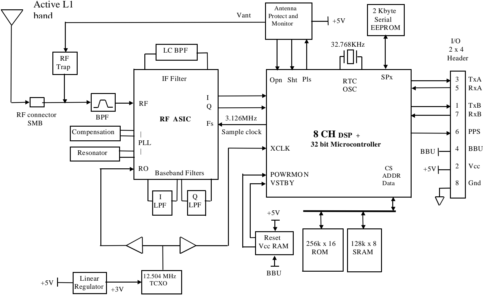
Figure 4-1. ACE II GPS Block Diagram
