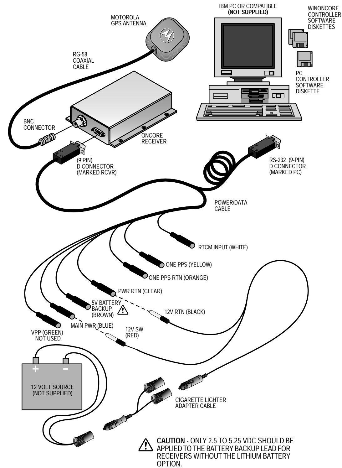
Figure QS-1 Oncore Evaluation Kit Setup
